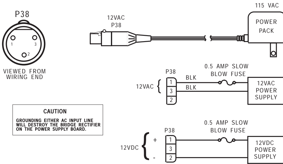
Fig. 5. Power Connections
